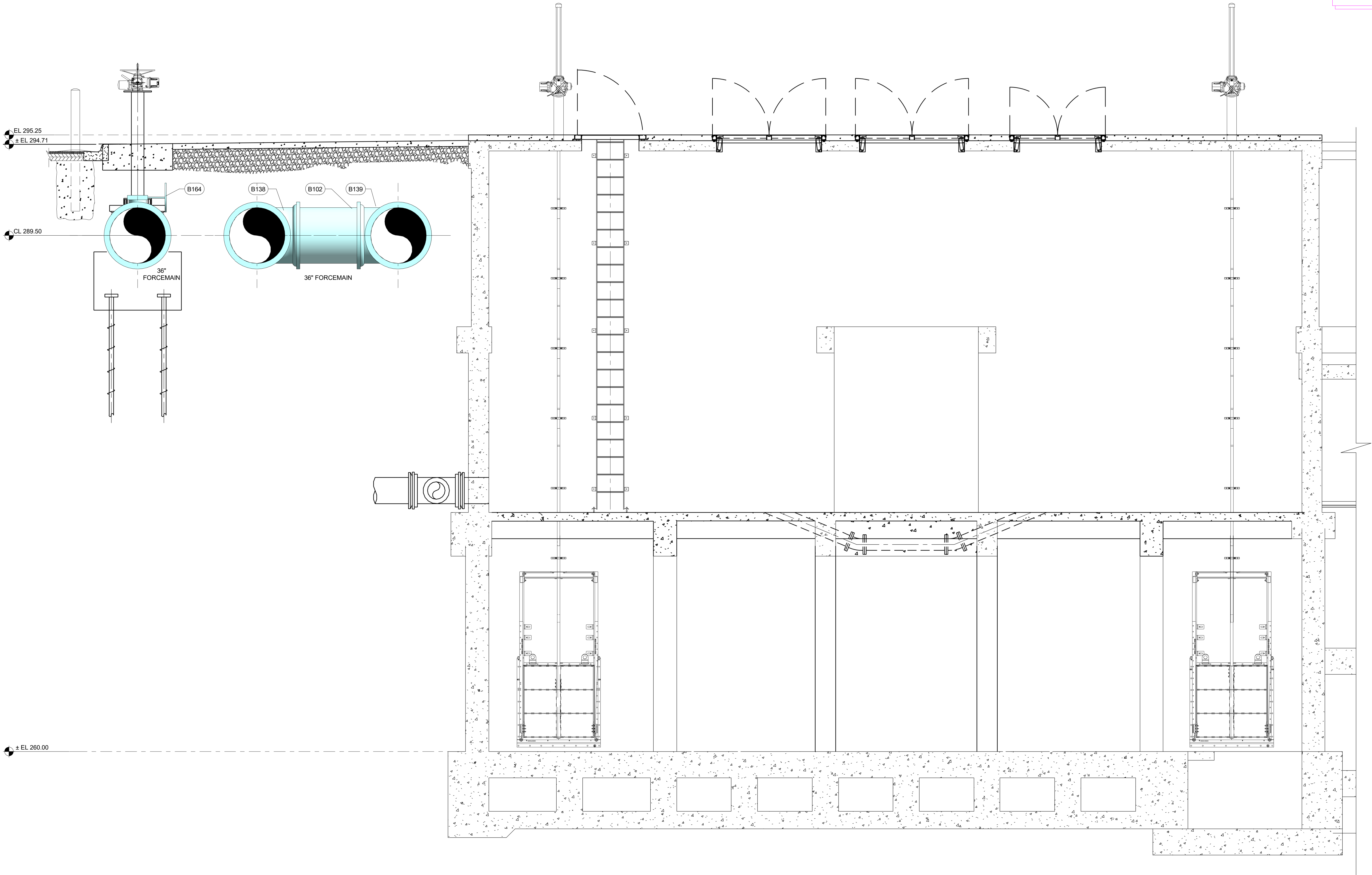
1 SECTION 3/8" = 1'-0" Ref: E/09-D304
