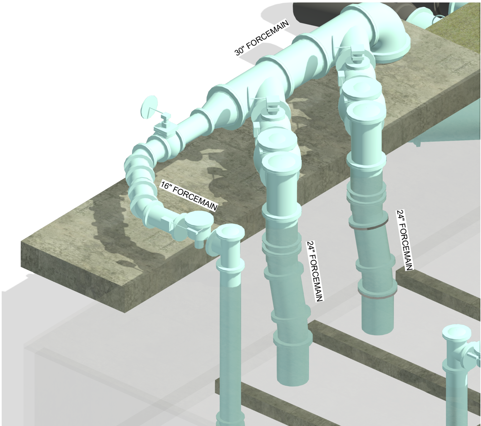
3 VIEW C & D
