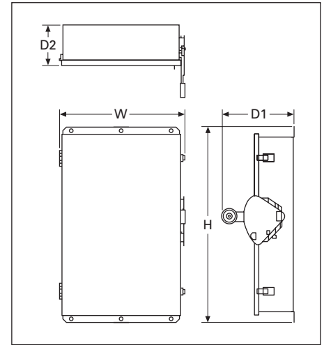
Figure 28.1-12. Shunt Trip Safety Switch, 240 Vac and 600 Vac
