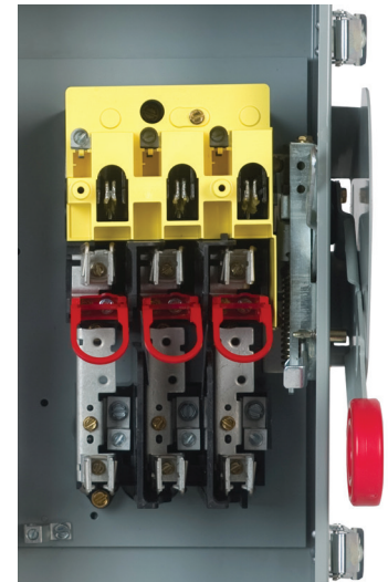
Enhanced Visible Blade
