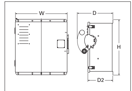
Figure 28.1-13. Auxiliary Power Heavy-Duty Safety Switch
